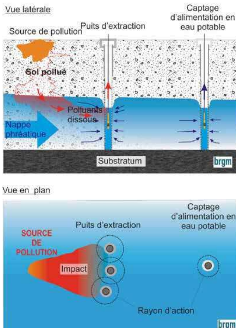
Figure 23. Example of active hydraulic trapping (pumping).
