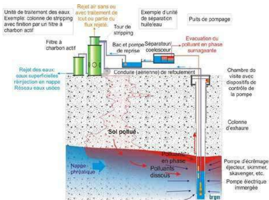
Figure 20. Schematic diagram of pumping skimming.
