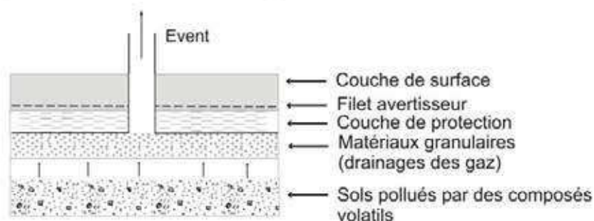
Figure 21. Example of different types of polluted site overlap.
