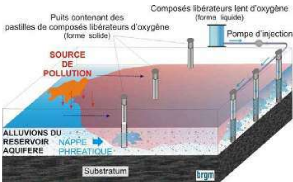
Figure 25. Schematic diagram of dynamic in situ biodegradation.
