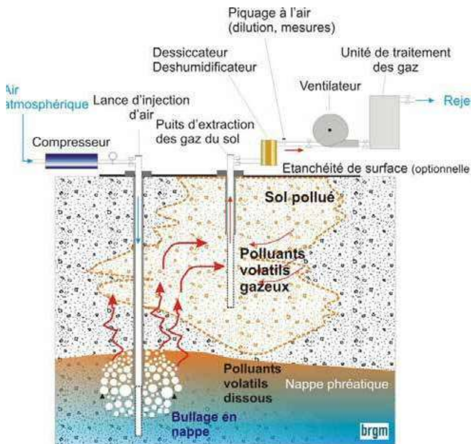
Figure 18. Schematic diagram of the bubbling coupled with the ventilation.
