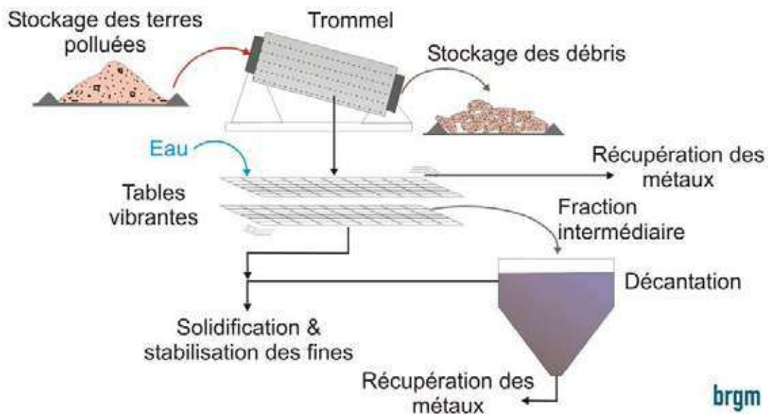
Figure 31. Schematic diagram of granulometric sorting.
