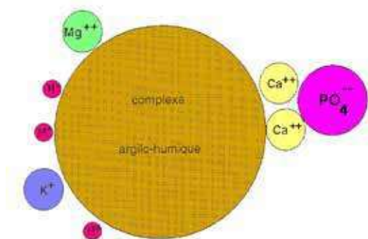
Figure 97. Fixing of ions on the clay-humic complex.
