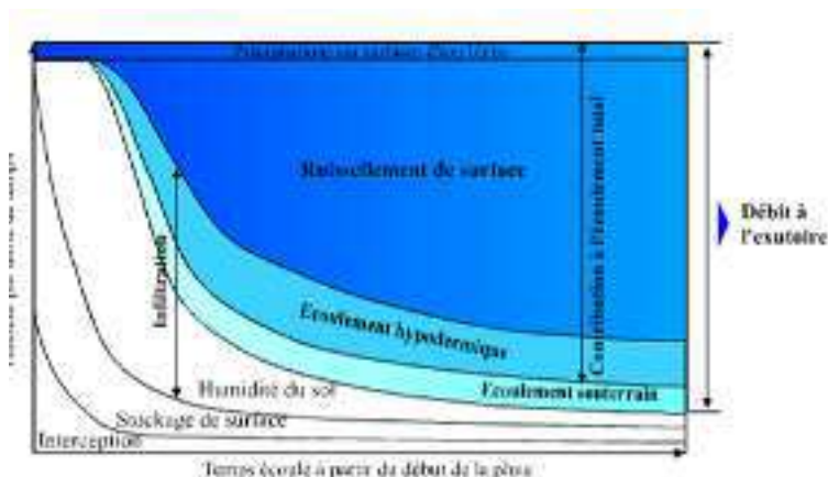
Figure 105. Repartition of precipitation height during a constant intensity showers. Source: Remanieras cited by Musy (2005)
