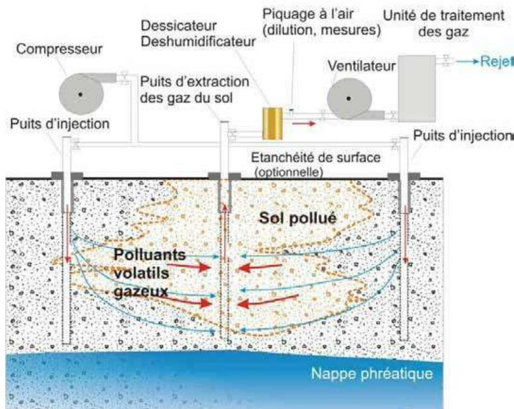
Figure 16. Schematic diagram of ventilation.
