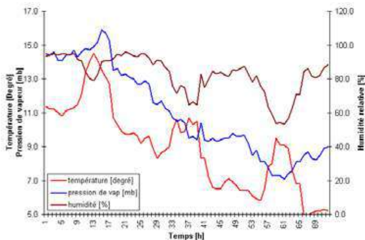
Figure 46. Evolution of temperature, vapour pressure and relative humidity.
