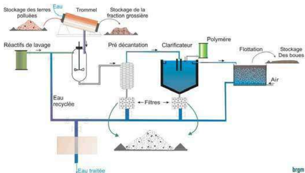
Figure 32. Schematic diagram of ex situ washing.
