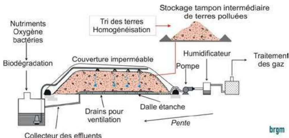
Figure 34. Schematic diagram of the biopile.
