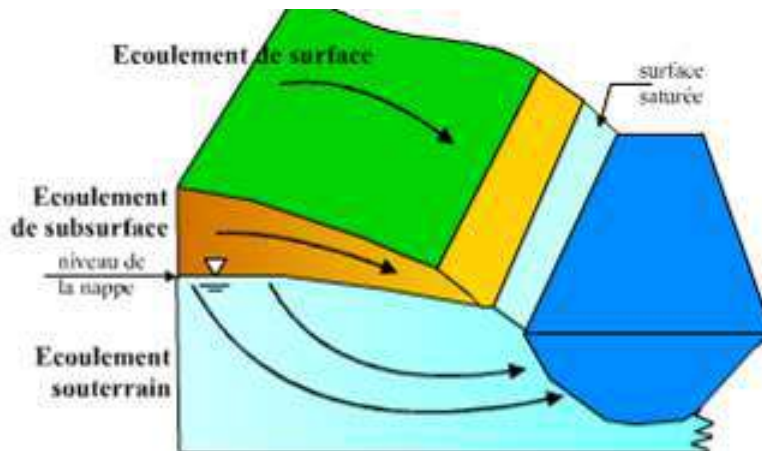
Figure 103. Different types of flow. Source: Musy (2005)
