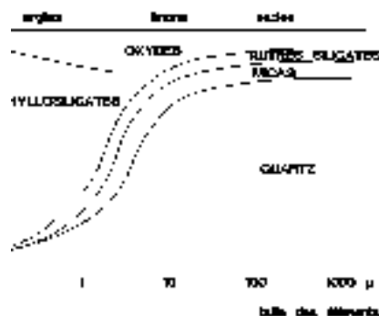
Figure 95. Mineralogical nature and size of the soil particles.
