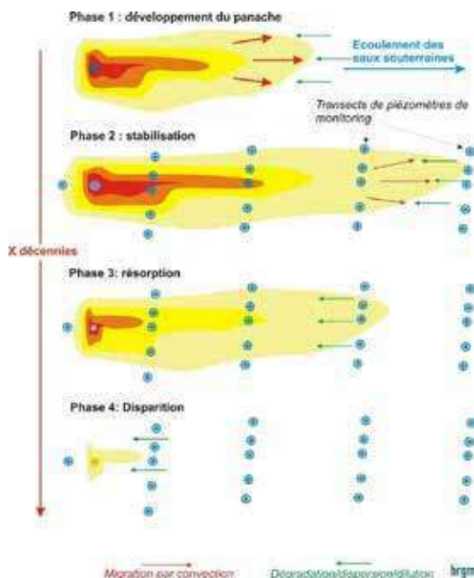
Figure 28. Life cycle of a plume subjected to natural attenuation.
