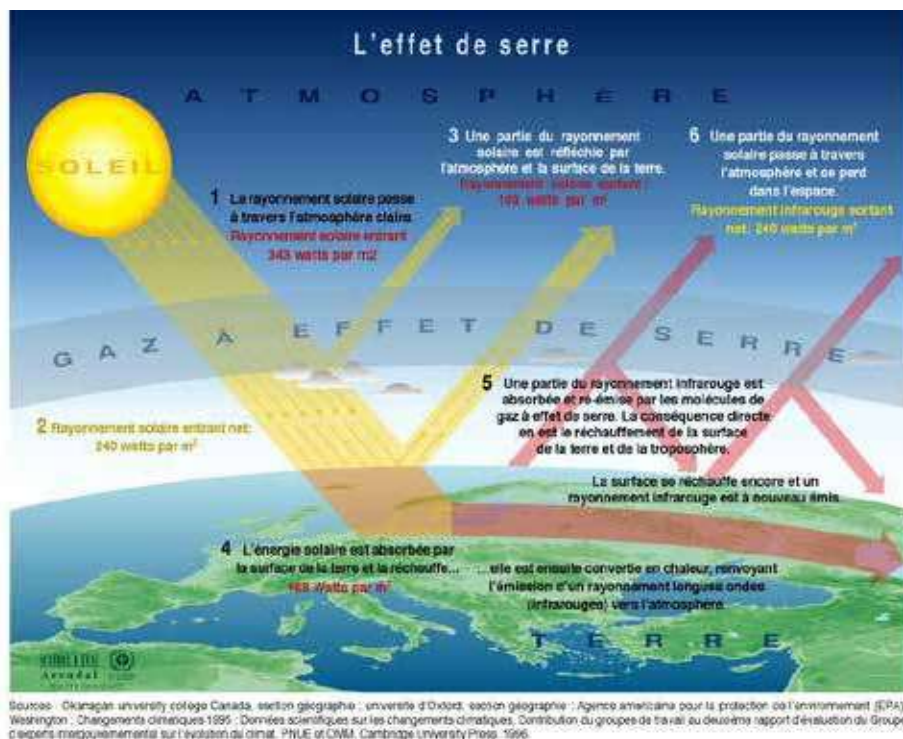
Figure 41. Greenhouse effect
