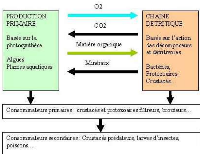
Figure 12. Matter Cycle and food pyramid. Source: haliosphere.over-blog.com
