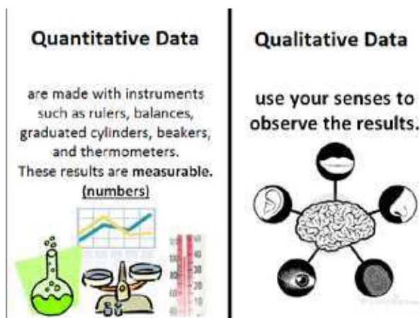
Figure 49. Quantitative data vs Qualitative data.
