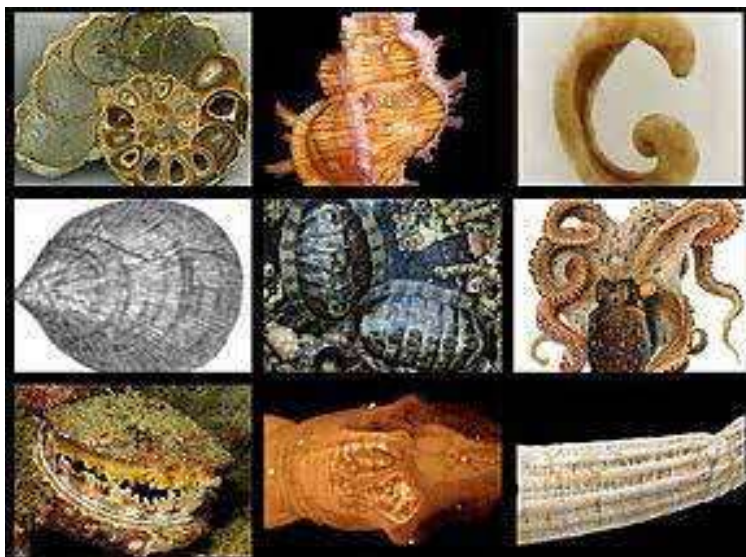
Figure 81. Examples of different classes of molluscs.
