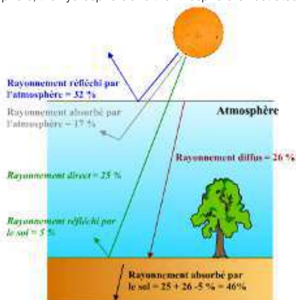
Figure 44. Action of solar radiation on the atmosphere, hydrosphere and lithosphere
