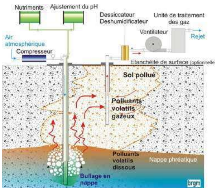
Figure 27. Schematic diagram of biosparging.
