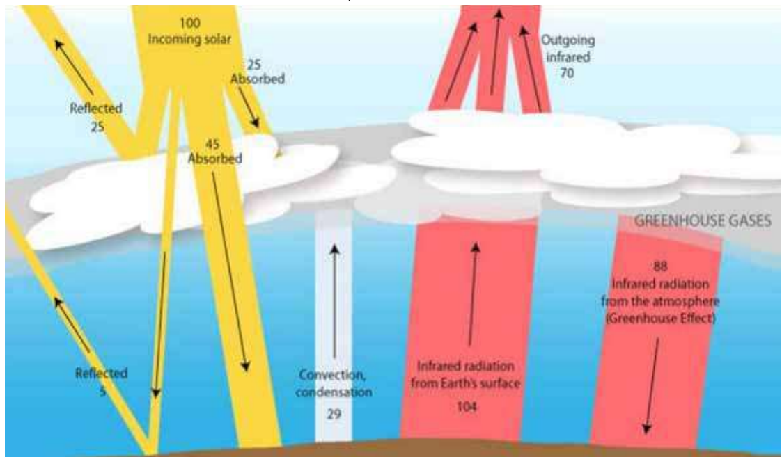
Figure 10. Radiative balance of the earth.
