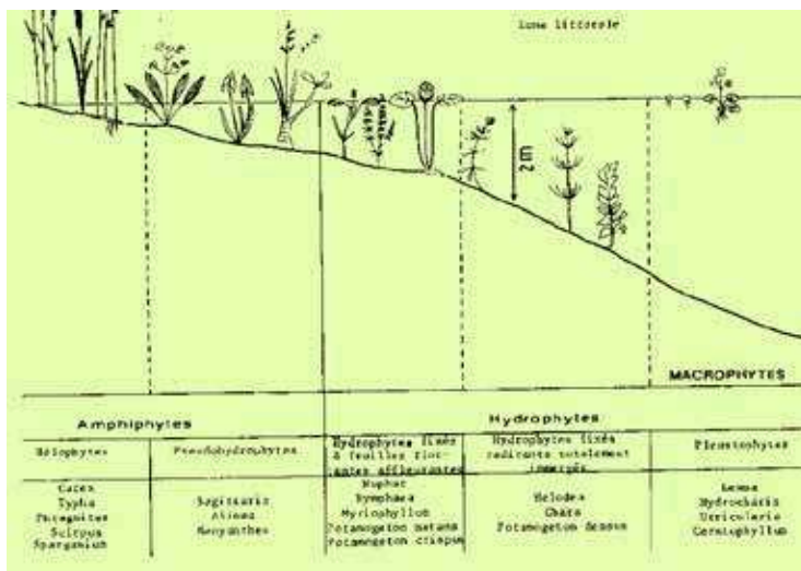
Figure 14. Distribution of plants in a stagnant water system. Source: Radoux (1999)
