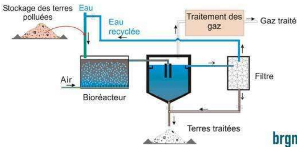
Figure 33. Schematic diagram of a bioreactor.
