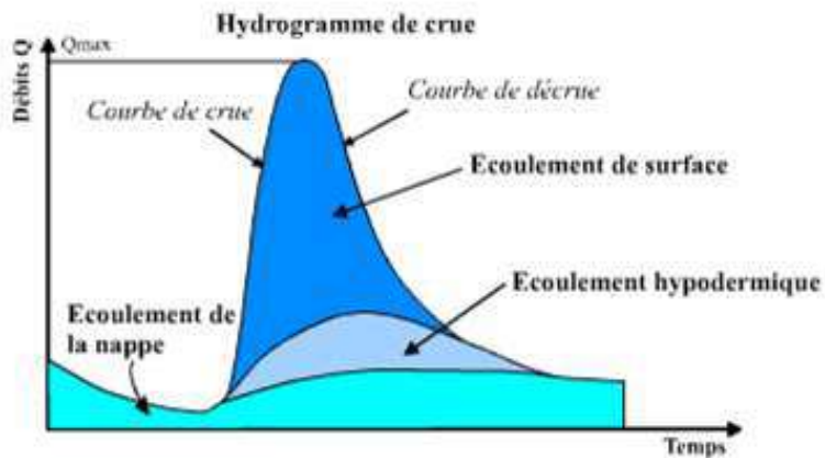
Figure 104. Breakdown of different phases of a flood hydrograph. Source: Musy (2005)
