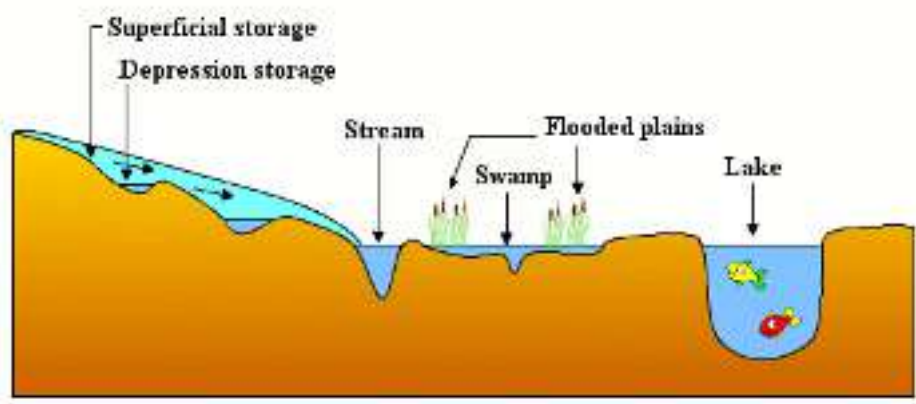
Figure 101. Surface water storage.
