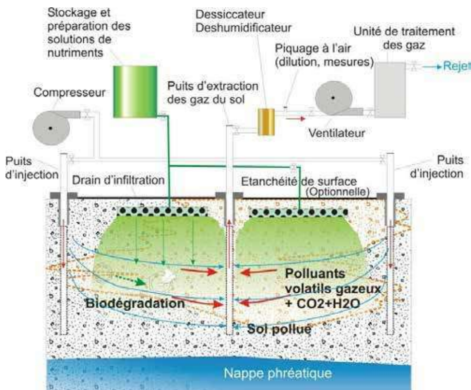
Figure 26. Diagram of the principle of bioventing.
