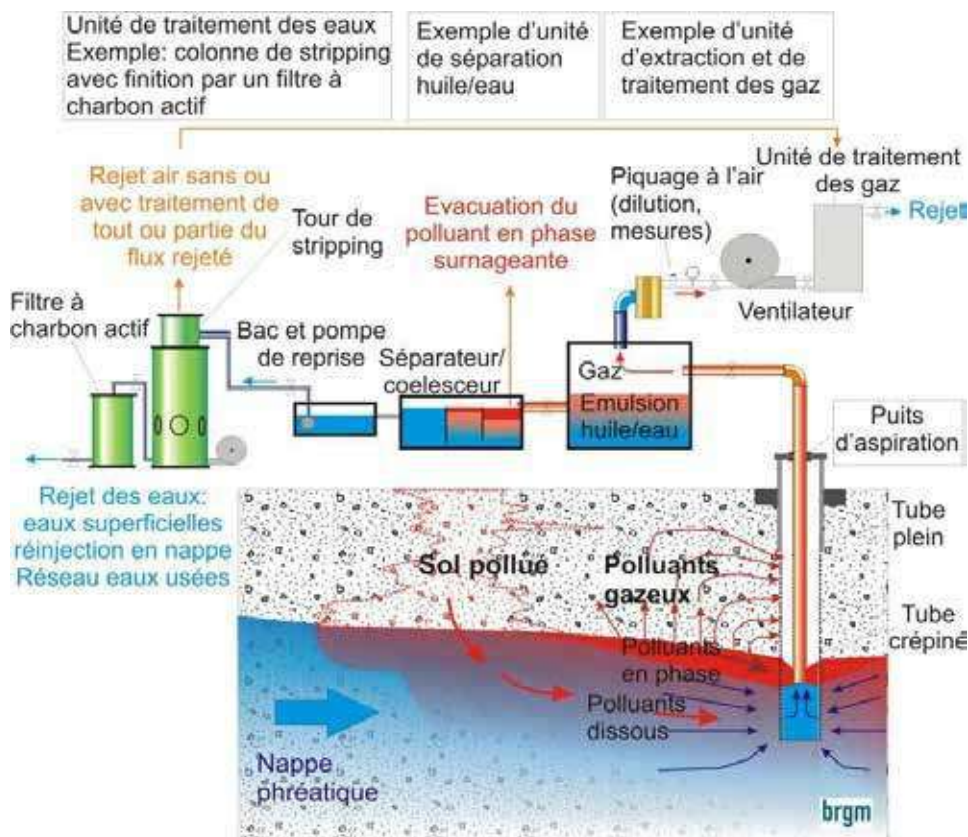
Figure 17. Dual phase extraction principle diagram.
