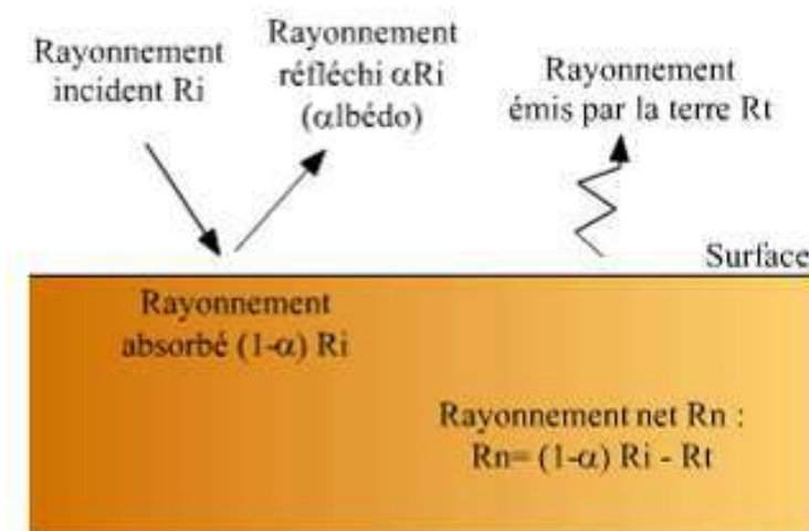
Figure 45. Balance of raditive exchange at the soil surface.
