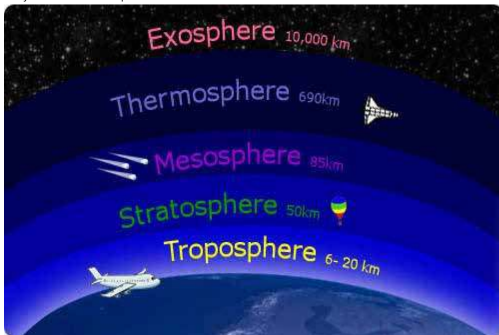
Figure 1. Layers of the atmosphere
