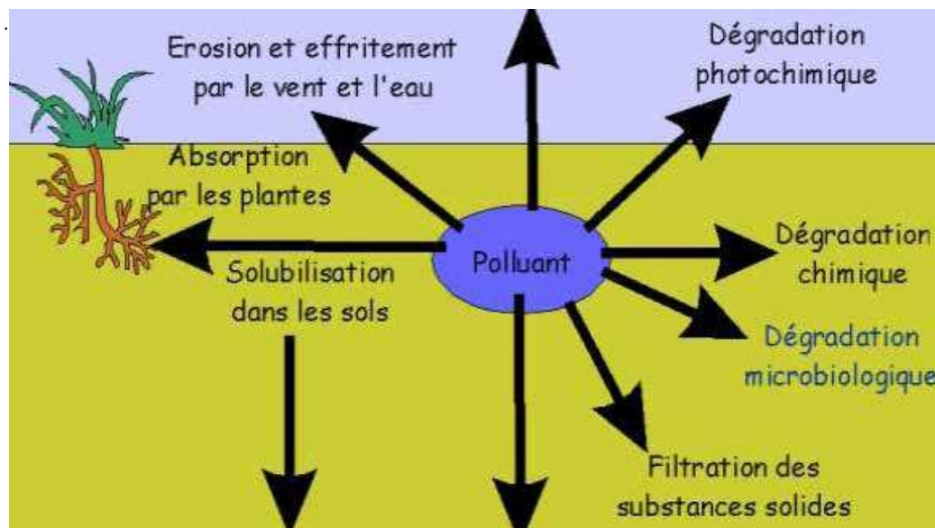
Figure 15 a + b. Fate of pollutants in soil.
