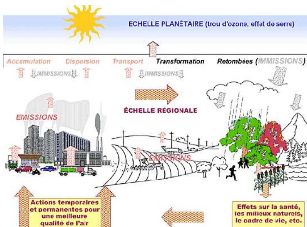
Figure 5. Cycle of pollutants in the atmosphere
