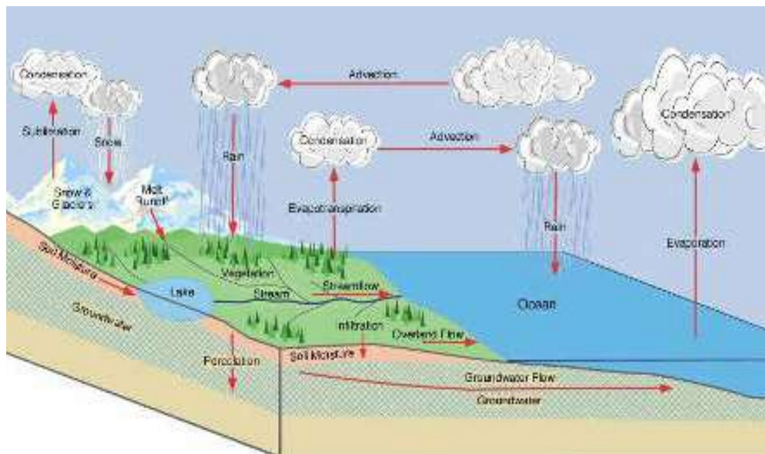
Figure 2. The hydrologic cycle. Source: Pidwirny (2006)
