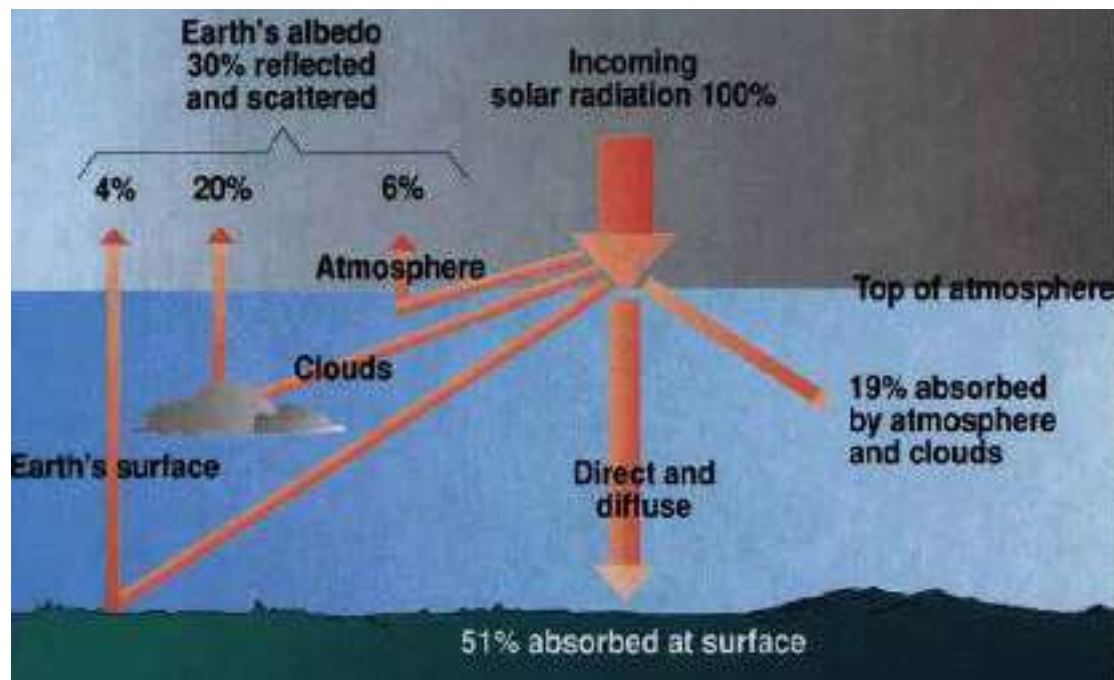
Figure 6. Radiation components.
