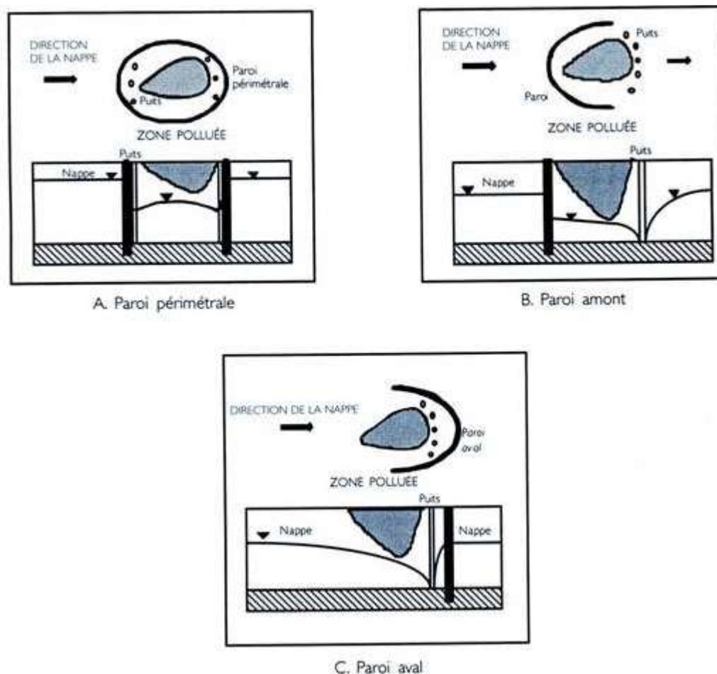
Figure 22. Example of vertical containment associated with pumping
