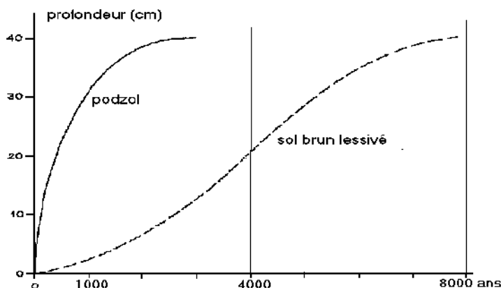
Figure 96. Trend rate of two soils type under atlantic climate.
