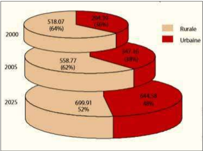
Figure 111. Trends in urbanization rates in Africa.
