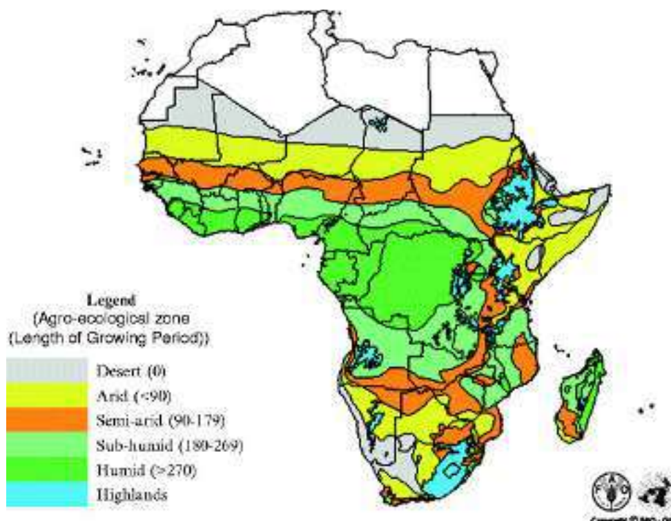
Figure 99. Main agro-ecological zones in sub-Saharan Africa.
