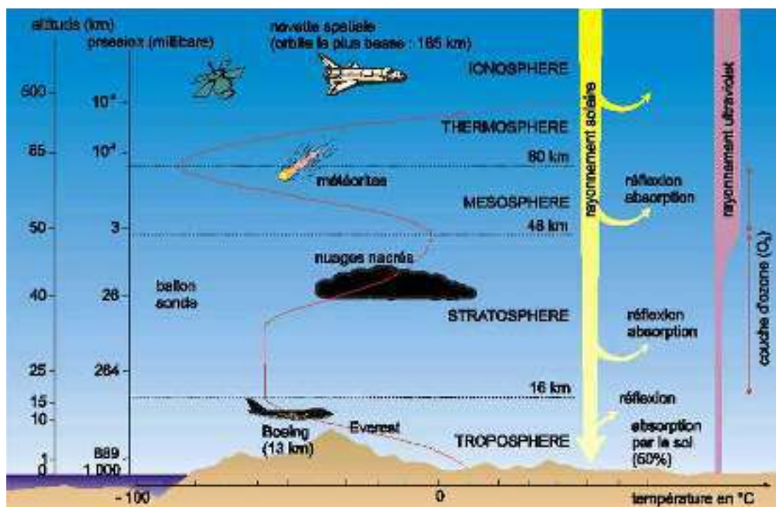
Figure 3. Variation of altitude, temperature and pressure as a function of atmospheric layers.
