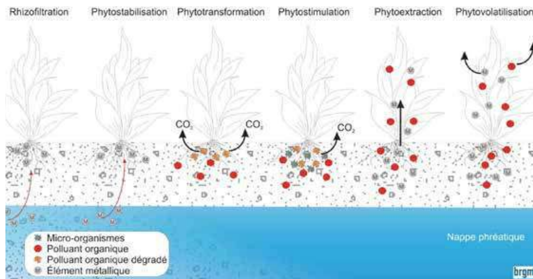
Figure 29. Examples of different types of phytoremediation.
