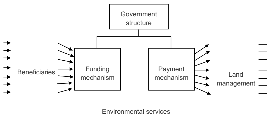
Figure 108. Structure of PES mechanisms.
