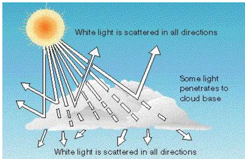
Figure 7. Lorenz-mie scattering for large particles (droplets).
