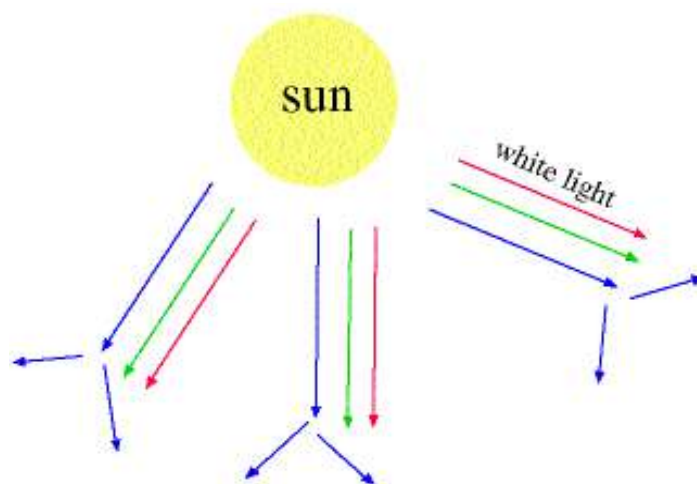
Figure 8. Rayleigh scattering for small particles (gas molecules).
